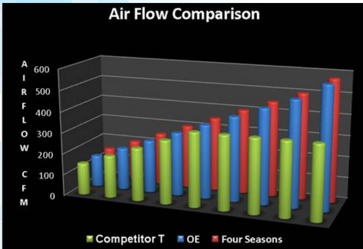
Airflow measured in CFM (Cubic Feet per Minute) Testing supplied by Unimotor, LTD.
